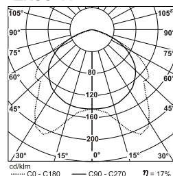
2x55 W
